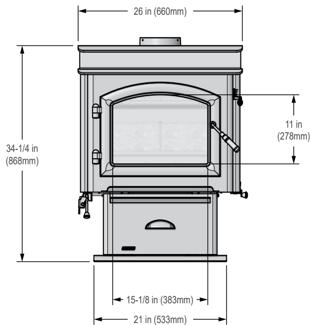
Figure 10.1 - Front View
