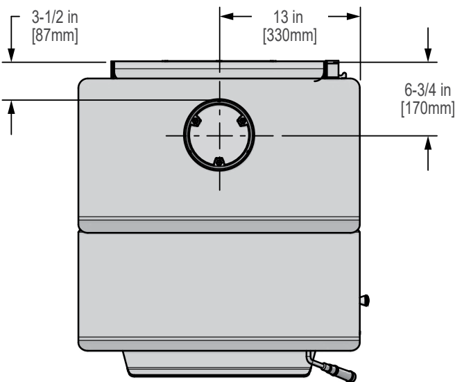
Figure 10.3 - Top View
