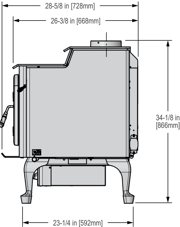
Figure 11.2 - Side View
