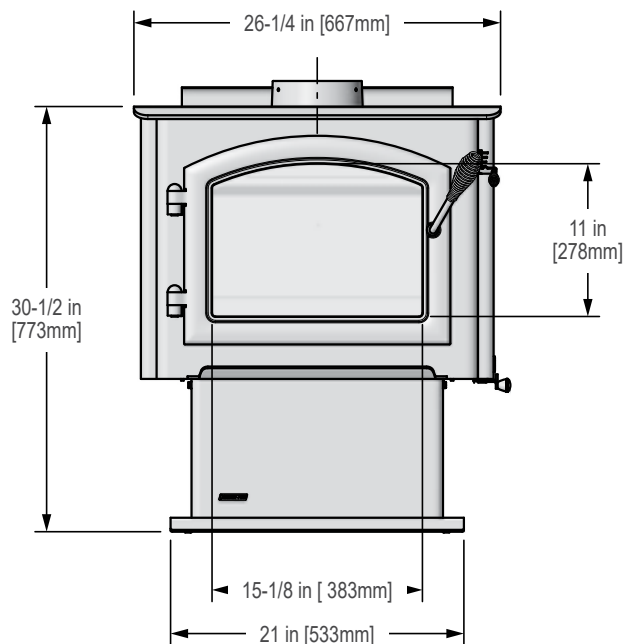
Figure 9.1 - Front View
