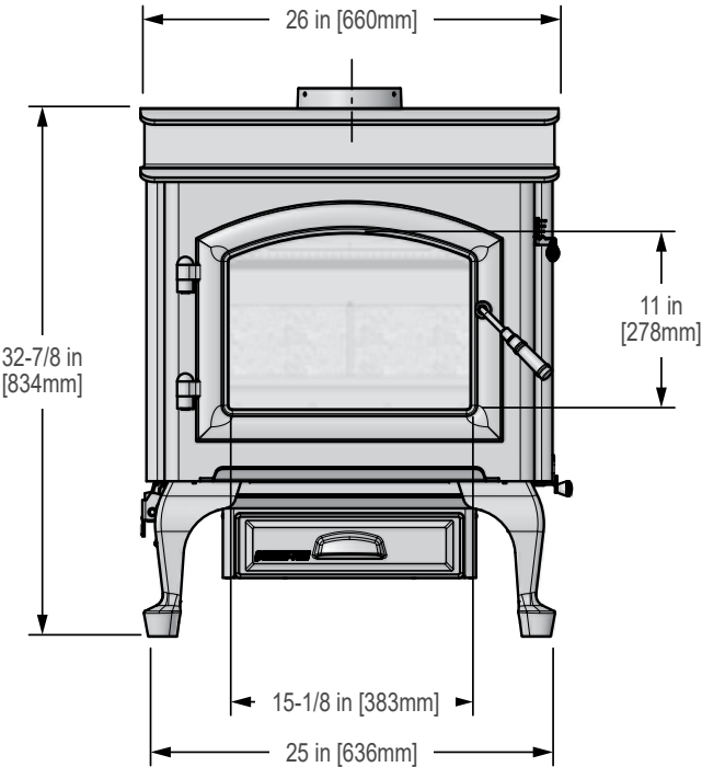
Figure 11.1 - Front View
