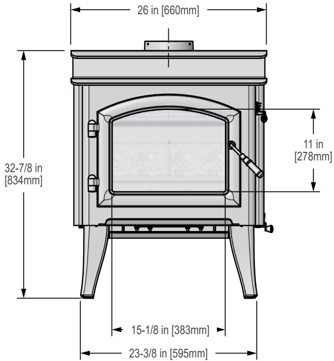
Figure 12.1 - Front View
